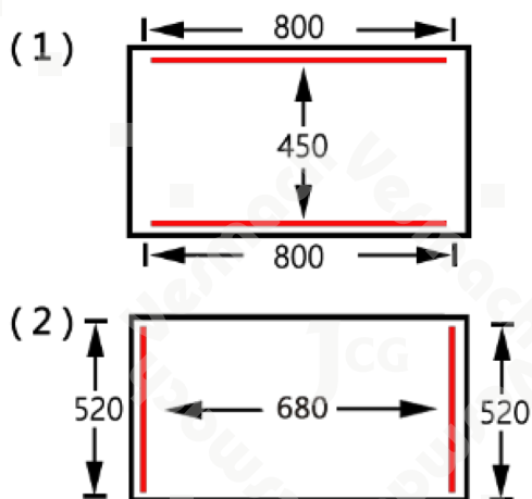
Diagrams of sealing beams position
